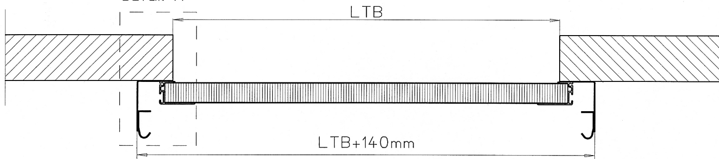
Detail "A"
